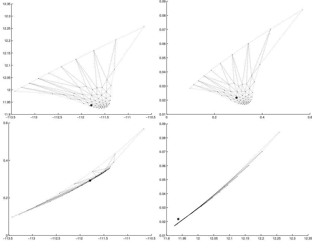
Figure 5. Triangulated ephemerides for 2003 BH_{84} . Top left: (-\alpha, \delta) plane; top right: (-\dot{\alpha}, \dot{\delta}) plane; bottom left: (-\alpha, -\dot{\alpha}) plane; bottom right: (\delta, \dot{\delta}) plane. Angles are in degrees and angular velocities are in degrees per day.
