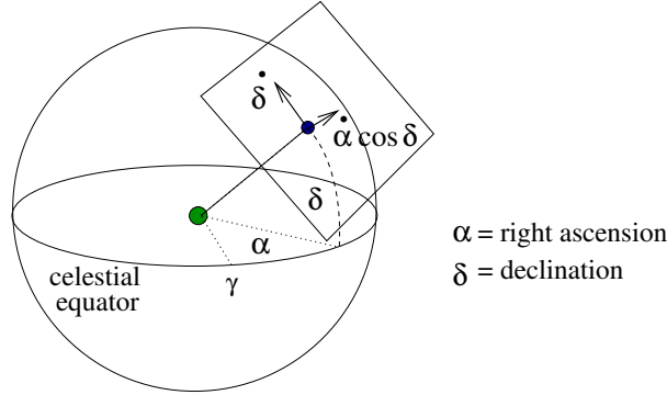
Figure 2. The celestial sphere and the components of an attributable.
