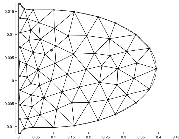
Figure 4. The AR for the asteroid 2003 BH_{84} : on the horizontal axis we plot f(r) = 1 - e^{-r^2/(2s^2)} , where s = \max(r) , in AU on the vertical axis we plot \dot{r} in AU/day. The real position of the asteroid ( r \approx 1.9834 , \dot{r} \approx 0.0066 ) is marked with a plus.
