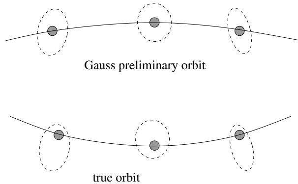
Figure 1. Qualitative sketch in which the orbit given by Gauss's method (preliminary orbit plus differential corrections) presents a curvature that is not reliable at all.
