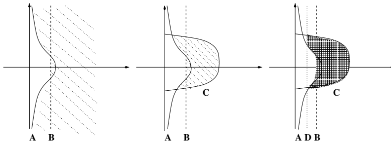
Figure 3. Qualitative sketch of an admissible region: it is defined by condition [(\mathbf{A}) \cup (\mathbf{B})^c] \cap (\mathbf{C}) \cap (\mathbf{D}) .
